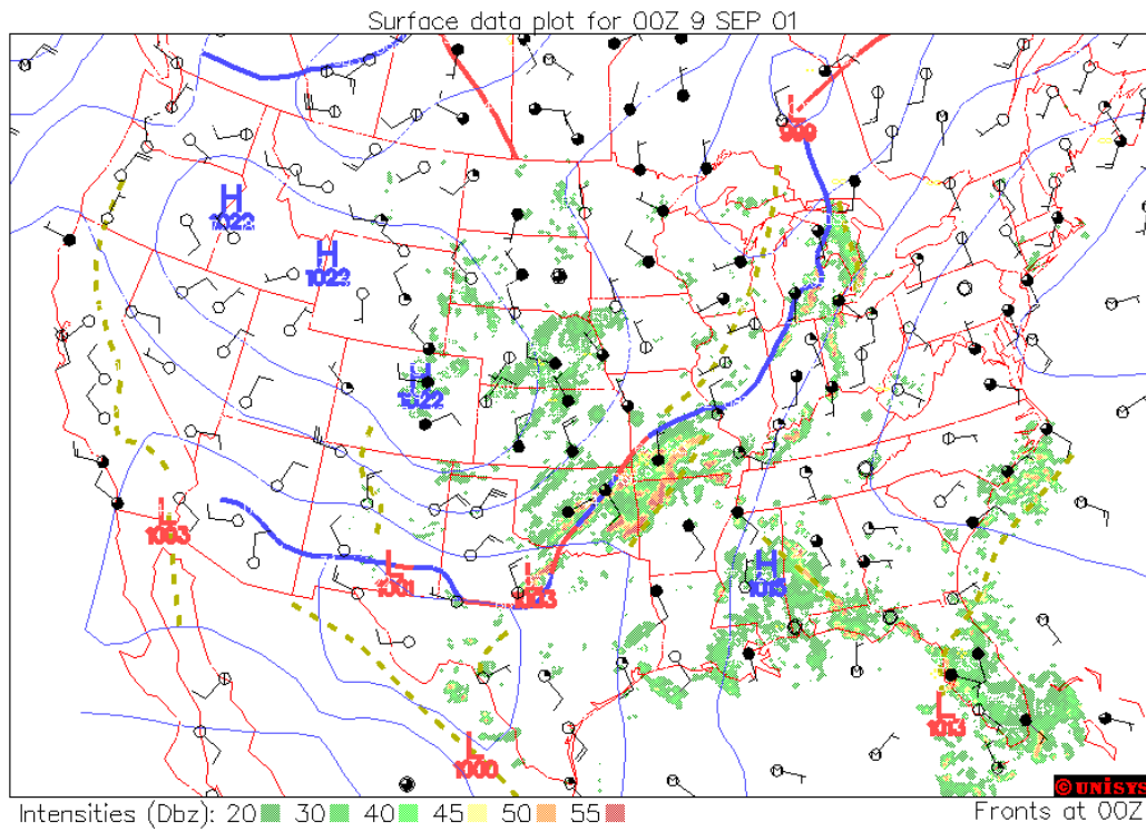
Figure 10 WEATHER MAP FOR SEPTEMBER 9, 2001
