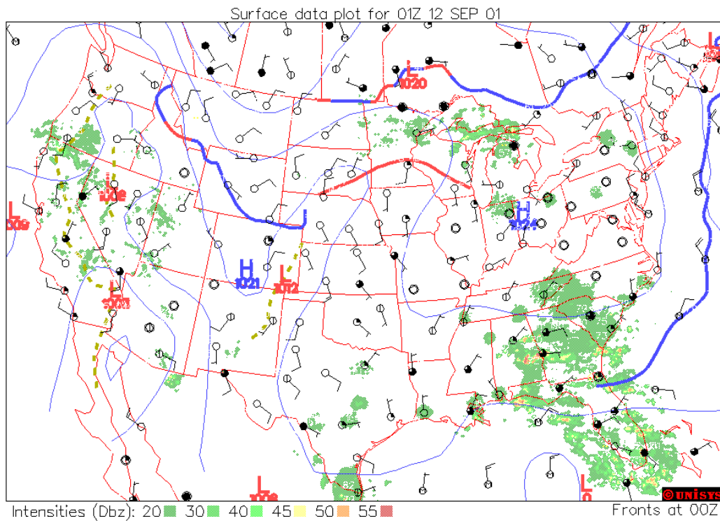
WEATHER MAP FOR SEPTEMBER 12, 2001
